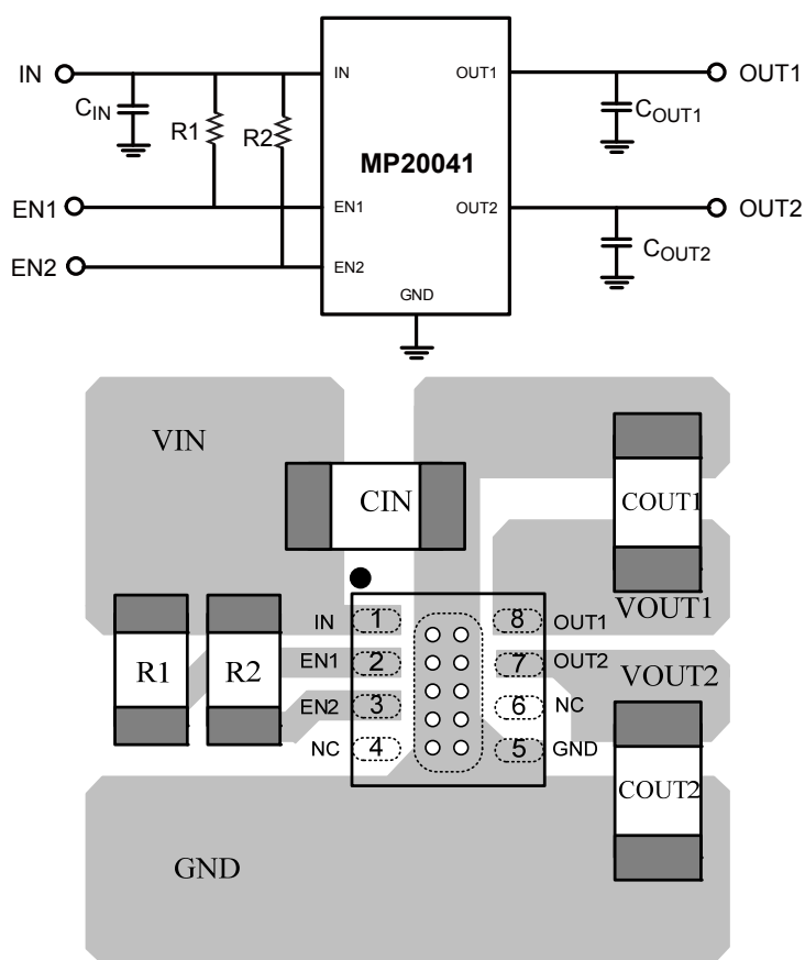
Top Layer Figure 5—PCB Layout
